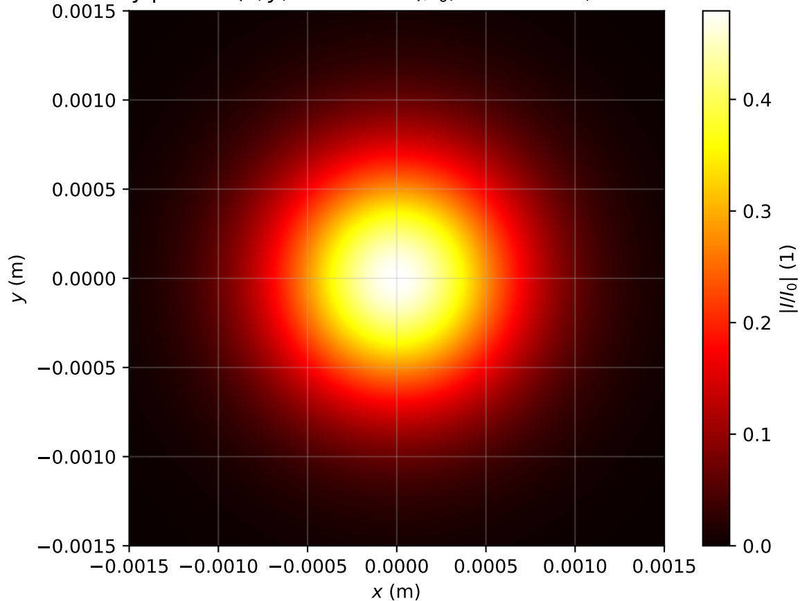
Intensity profile I(x, y, z = 3.025m)/I_0 , \text{Pin}=0.4\text{Pcr} , artificial time
